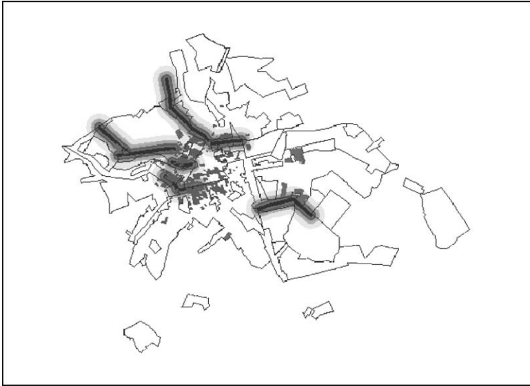
Fig. 3. Overlay and spatial independence of factors determining the transition from residential to mixed use ( RES_MIX ). The buffer bands are distance to planned roads ( plan_rds ), the darker diffused spots are areas of medium-high density of occupation ( mh_dens ), and the darker polygons correspond to social housing ( soc_hous ).
