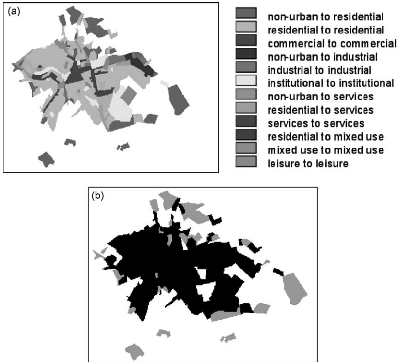
Fig. 2. (a) Land use change 1979–1988 (b) Non-urban to residential land use change ( NU_RES in grey) 1979–1988.
