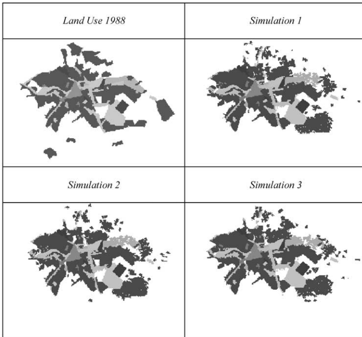
Fig. 5. The three best simulations compared to the actual land use in 1988. Leisure and recreation (very light grey), institutional (very dark grey), and the central commercial zone (mid grey) did not incur any transitions during the observed time period. The new mixed land use zone that emerged in the north-western part of the city was accurately modeled particularly in the first and third simulations.
