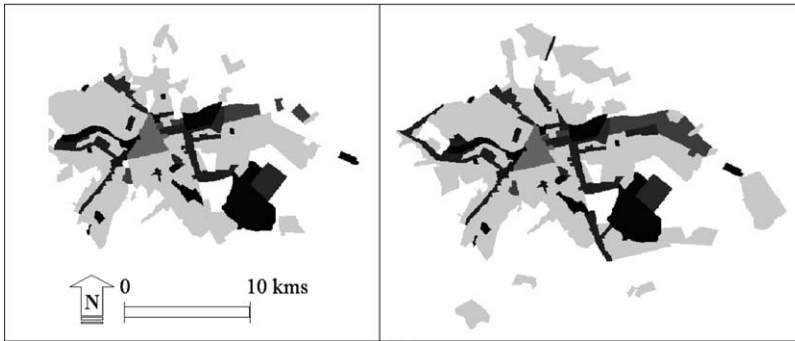
Fig. 1. Land use in Bauru in 1979 (left) and 1988 (right). Residential use is light grey, institutional use is black, service corridors and zones, and industrial uses are dark grey, and commercial use is mid grey.
