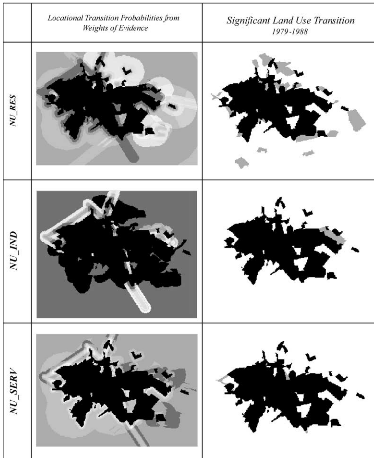
Fig. 4. Estimated transition probability surfaces and land use change 1979–1988 The range of probabilities runs from high (light grey) to low (dark grey) and the changes in land use are in light grey, existing land use in dark grey.
