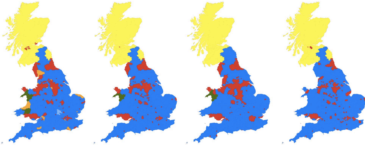
Figure 7: From left to right: ( B_P ) Prediction using the actual votes and the polls; ( C_P ) prediction by using the percolation and the occupational data; ( D_P ) prediction using solely the percolation; and ( E_P ) prediction using the occupational data.
